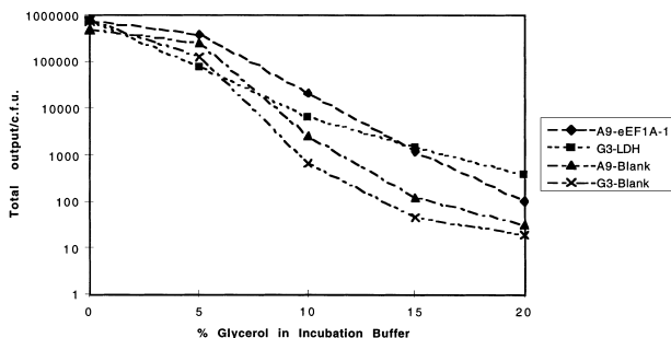
Fig. 5. Background assay to monitor the effect of glycerol on the number of phage particles sticking non-specifically to the antigen. Phage-ab G3 and A9 were added either to blank wells or to wells coated with 2 µg of the non-cognate antigen. Upon washing, phages were eluted and titered.
